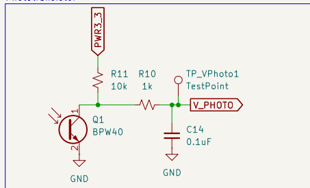
Phototransistor
